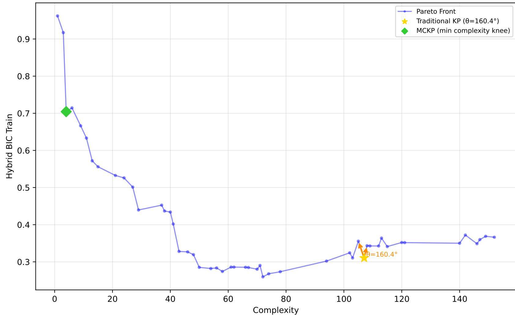
605_fri_c2_250_25 - Run 22 - MVP - Hybrid BIC Train \lambda_1=0.30, \lambda_2=0.00, \lambda_3=1.00 | Difficulty: 1.00 | Method: hmr
