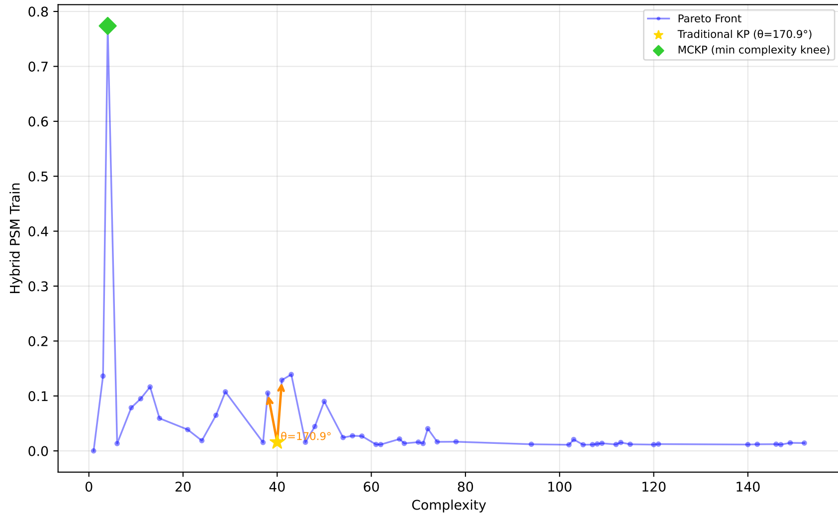
605_fri_c2_250_25 - Run 22 - SVP - Hybrid PSM Train \lambda_1=0.10, \lambda_2=0.00, \lambda_3=0.00 | Difficulty: 1.00 | Method: hmr
