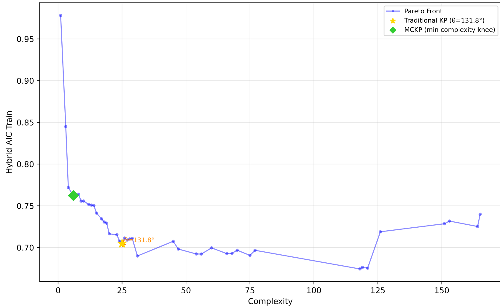
605_fri_c2_250_25 - Run 23 - MVP - Hybrid AIC Train \lambda_1=0.30, \lambda_2=0.00, \lambda_3=1.00 | Difficulty: 0.91 | Method: hmr
