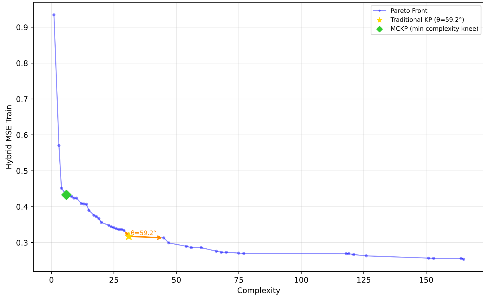
605_fri_c2_250_25 - Run 23 - MVP - Hybrid MSE Train \lambda_1=0.10, \bar{\lambda}_2=0.00, \bar{\lambda}_3=0.00 | Difficulty: 0.91 | Method: hmr
