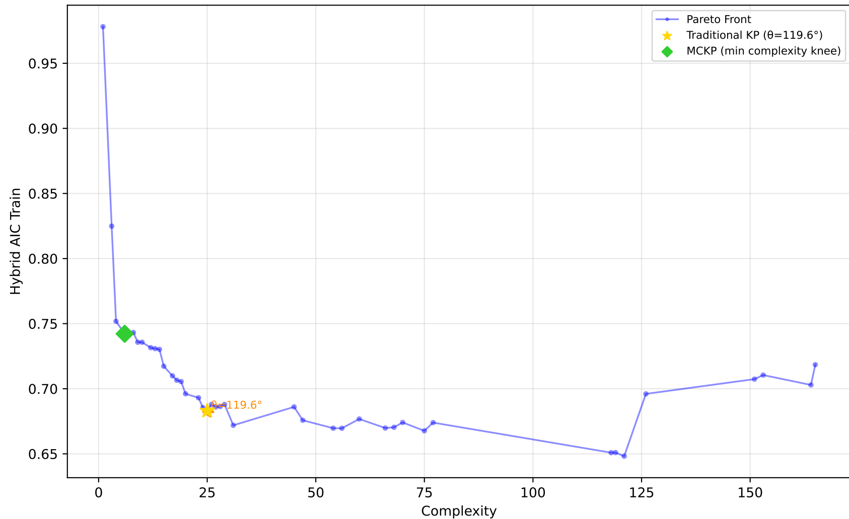
605_fri_c2_250_25 - Run 23 - SVP - Hybrid AIC Train \lambda_1=0.10, \lambda_2=0.00, \lambda_3=0.00 | Difficulty: 0.91 | Method: hmr
