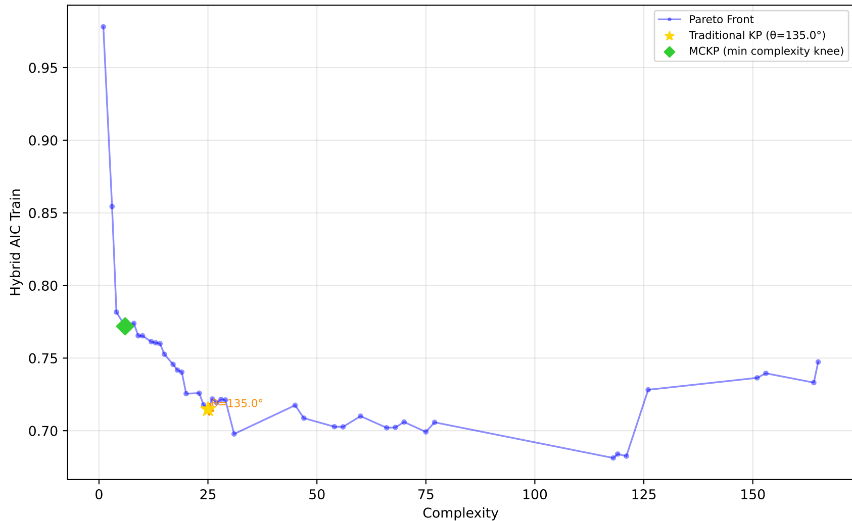
605_fri_c2_250_25 - Run 23 - SVP - Hybrid AIC Train \lambda_1=0.40, \lambda_2=0.00, \lambda_3=0.20 | Difficulty: 0.91 | Method: hmr
