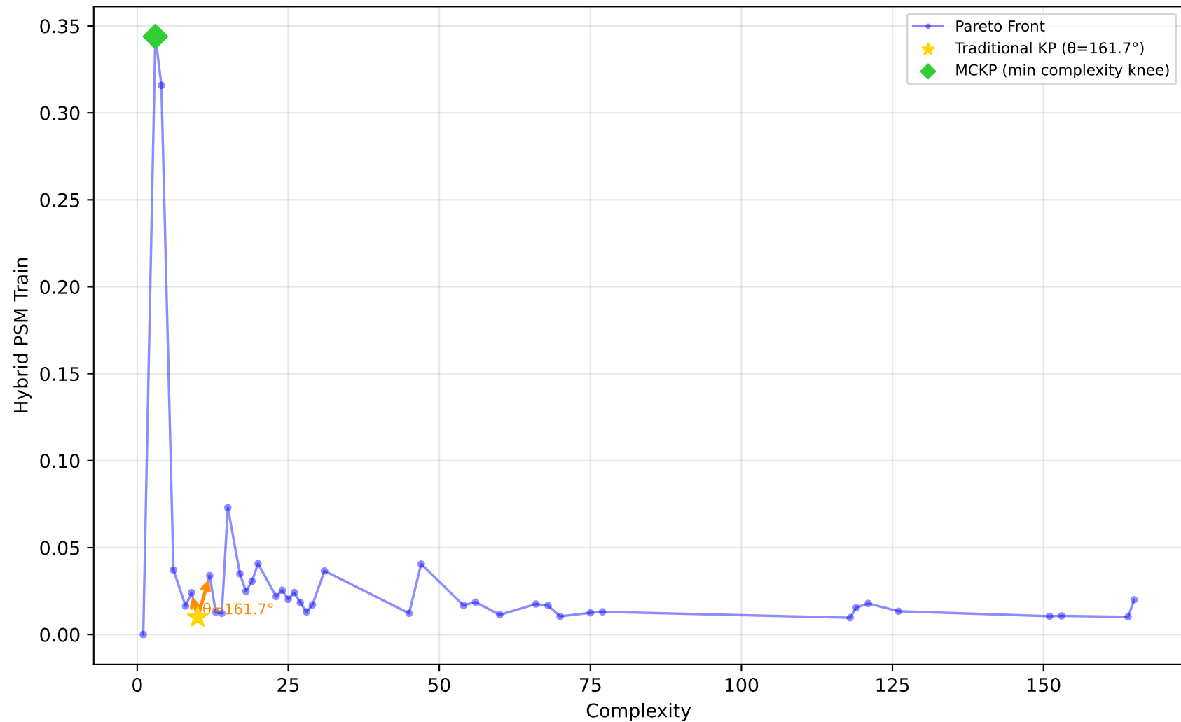
605_fri_c2_250_25 - Run 23 - SVP - Hybrid PSM Train \lambda_1=0.10, \lambda_2=0.00, \lambda_3=0.00 | Difficulty: 0.91 | Method: hmr
