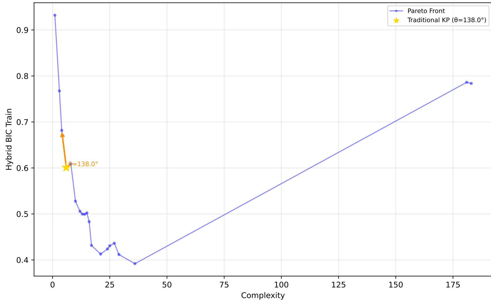
605_fri_c2_250_25 - Run 24 - MVP - Hybrid BIC Train \lambda_1=0.10, \lambda_2=0.00, \lambda_3=0.00 | Difficulty: 1.00 | Method: hmr
