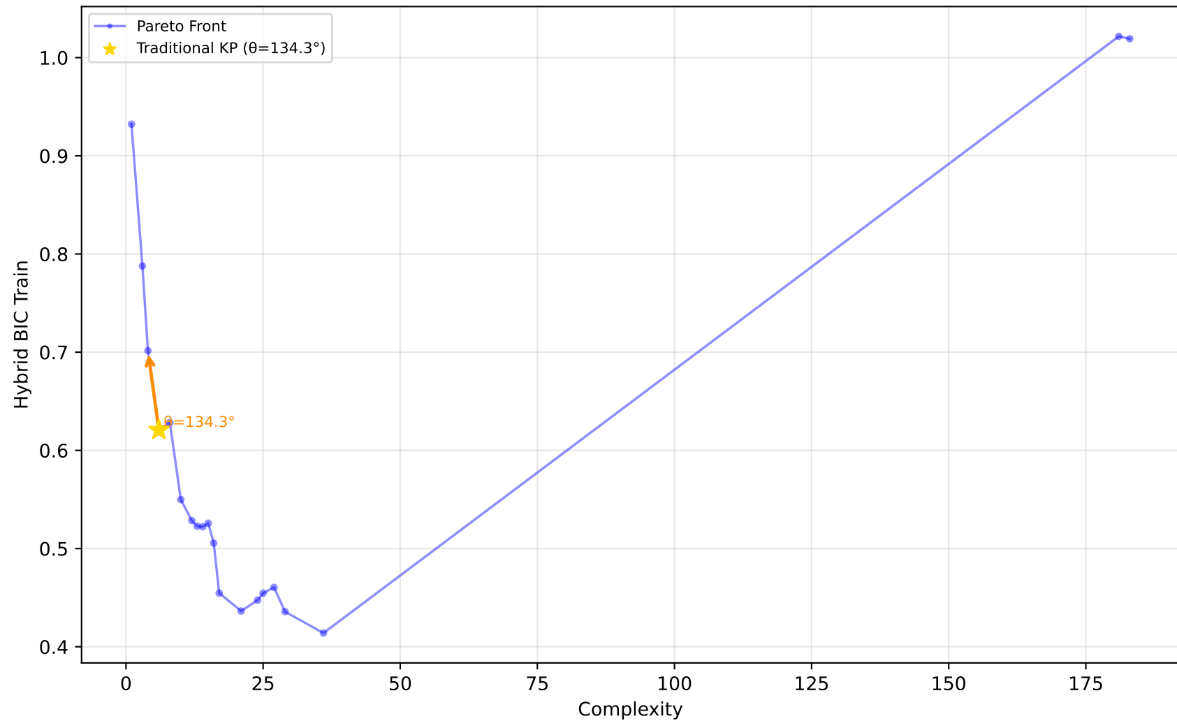
605_fri_c2_250_25 - Run 24 - MVP - Hybrid BIC Train \lambda_1=0.30, \lambda_2=0.00, \lambda_3=1.00 | Difficulty: 1.00 | Method: hmr
