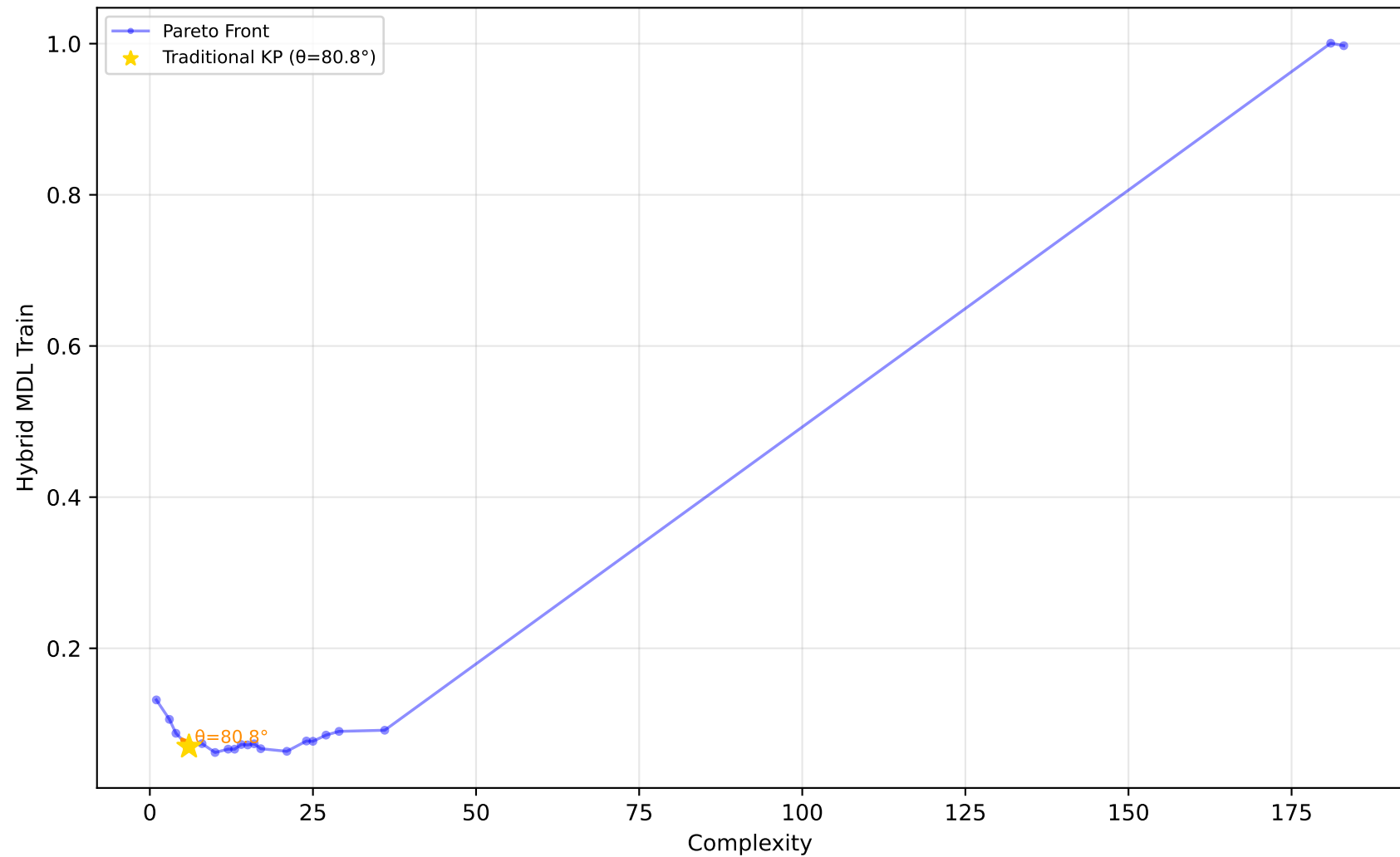
605_fri_c2_250_25 - Run 24 - MVP - Hybrid MDL Train \lambda_1=0.10, \bar{\lambda}_2=0.00, \bar{\lambda}_3=0.00 | Difficulty: 1.00 | Method: hmr
