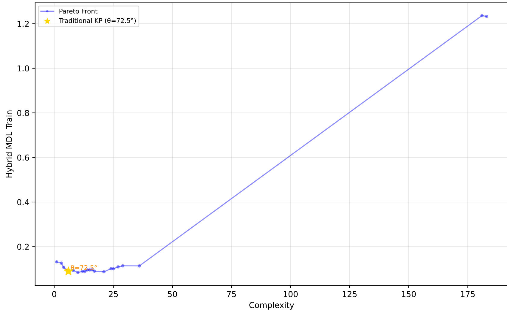
605_fri_c2_250_25 - Run 24 - MVP - Hybrid MDL Train \lambda_1=0.30, \bar{\lambda}_2=0.00, \lambda_3=1.00 | Difficulty: 1.00 | Method: hmr
