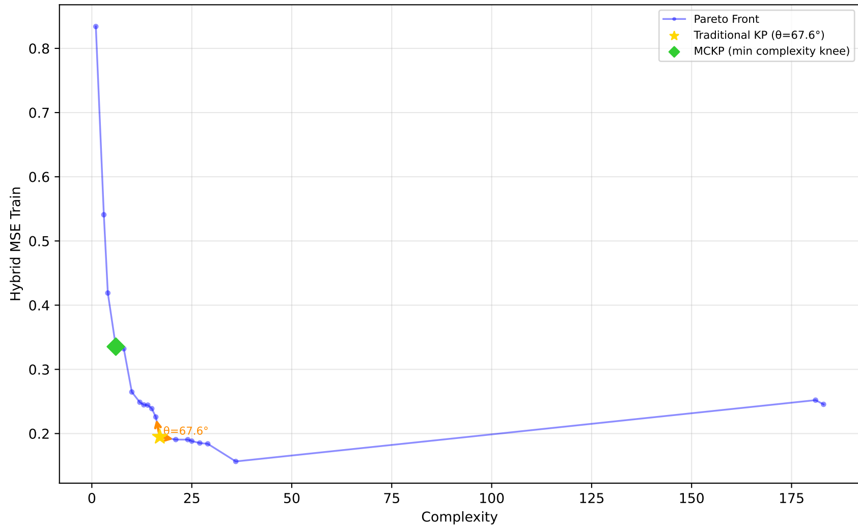
605_fri_c2_250_25 - Run 24 - MVP - Hybrid MSE Train \lambda_1=0.10, \bar{\lambda}_2=0.00, \bar{\lambda}_3=0.00 | Difficulty: 1.00 | Method: hmr
