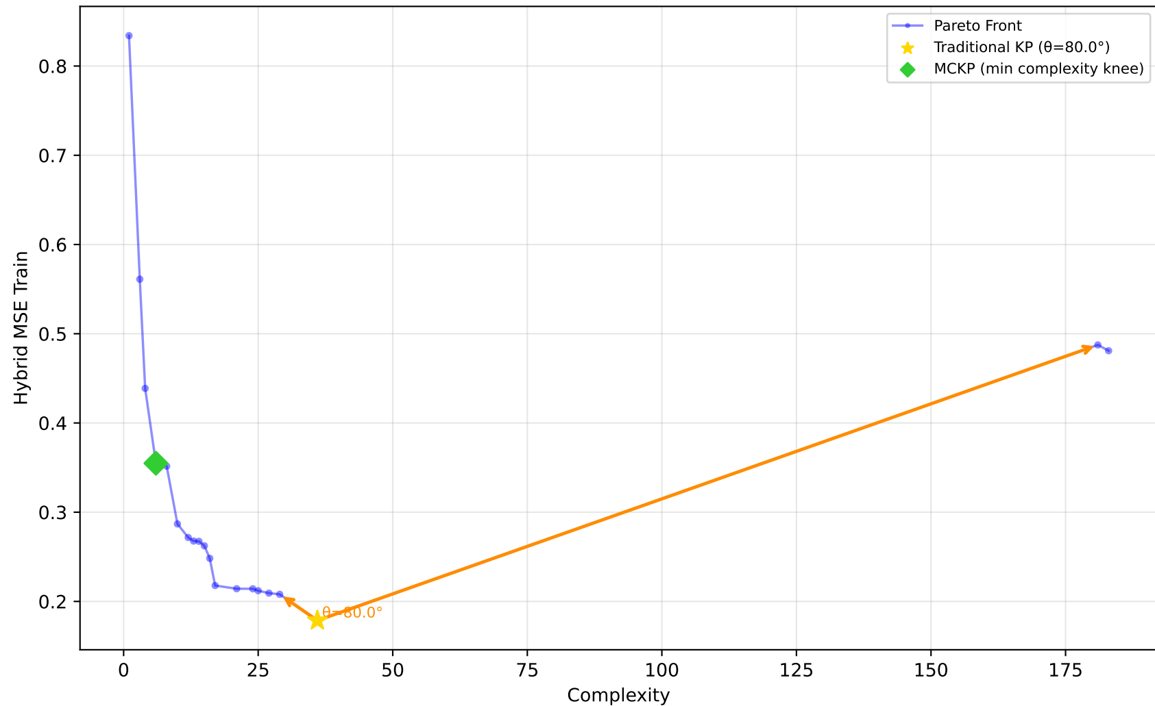
605_fri_c2_250_25 - Run 24 - MVP - Hybrid MSE Train \lambda_1=0.30, \lambda_2=0.00, \lambda_3=1.00 | Difficulty: 1.00 | Method: hmr
