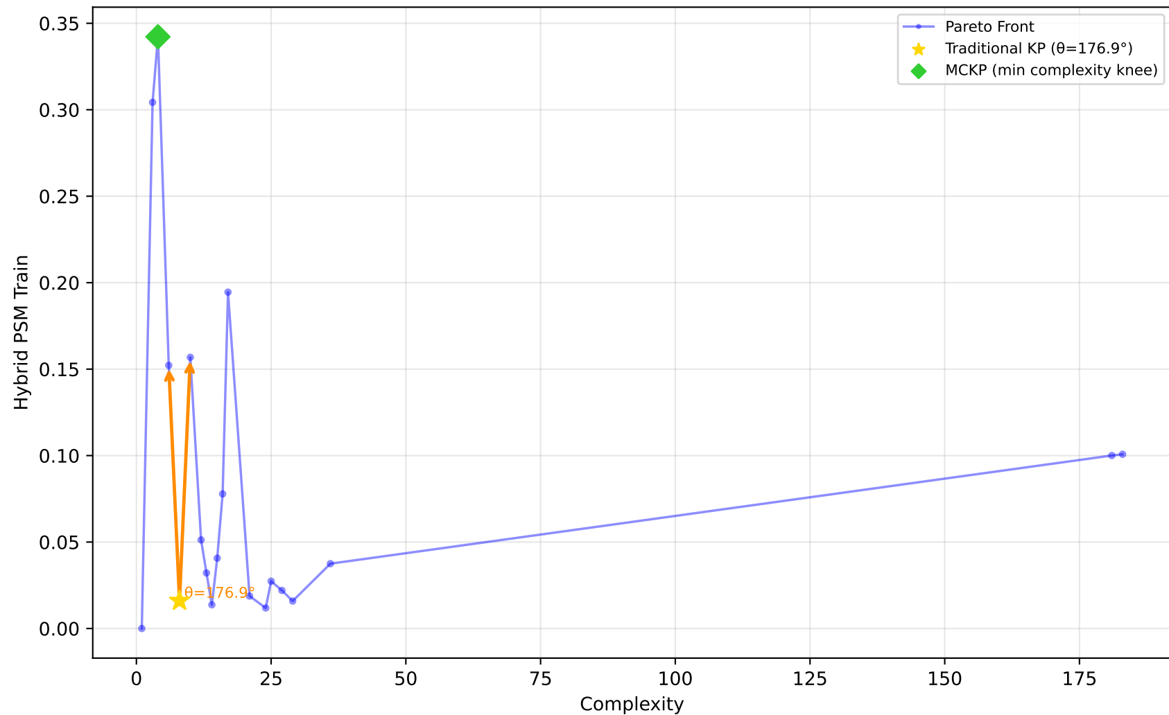
605_fri_c2_250_25 - Run 24 - MVP - Hybrid PSM Train \lambda_1=0.10, \lambda_2=0.00, \lambda_3=0.00 | Difficulty: 1.00 | Method: hmr
