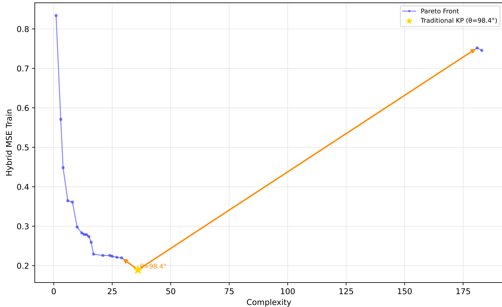
605_fri_c2_250_25 - Run 24 - SVP - Hybrid MSE Train \lambda_1=0.40, \lambda_2=0.00, \lambda_3=0.20 | Difficulty: 1.00 | Method: hmr
