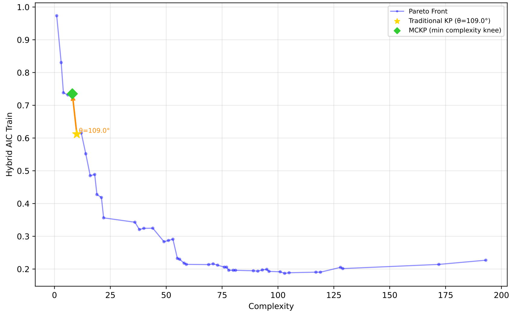
605_fri_c2_250_25 - Run 25 - MVP - Hybrid AIC Train \lambda_1=0.10, \lambda_2=0.00, \lambda_3=0.00 | Difficulty: 1.00 | Method: hmr
