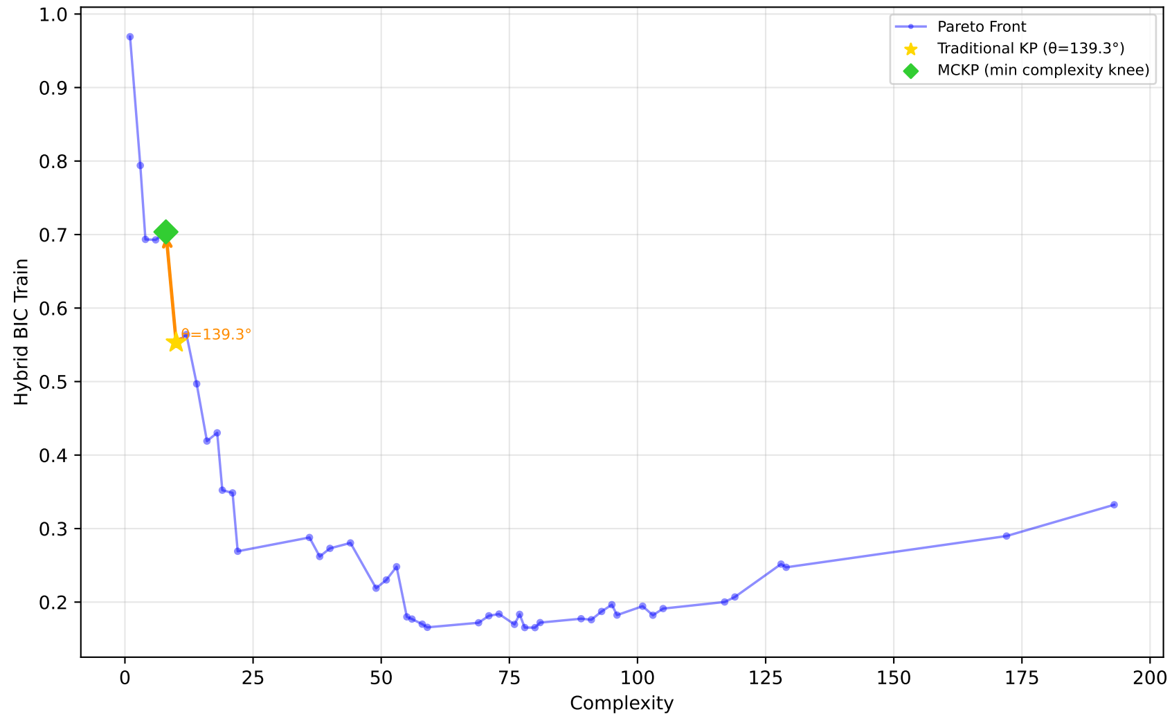
605_fri_c2_250_25 - Run 25 - MVP - Hybrid BIC Train \lambda_1=0.10, \lambda_2=0.00, \lambda_3=0.00 | Difficulty: 1.00 | Method: hmr
