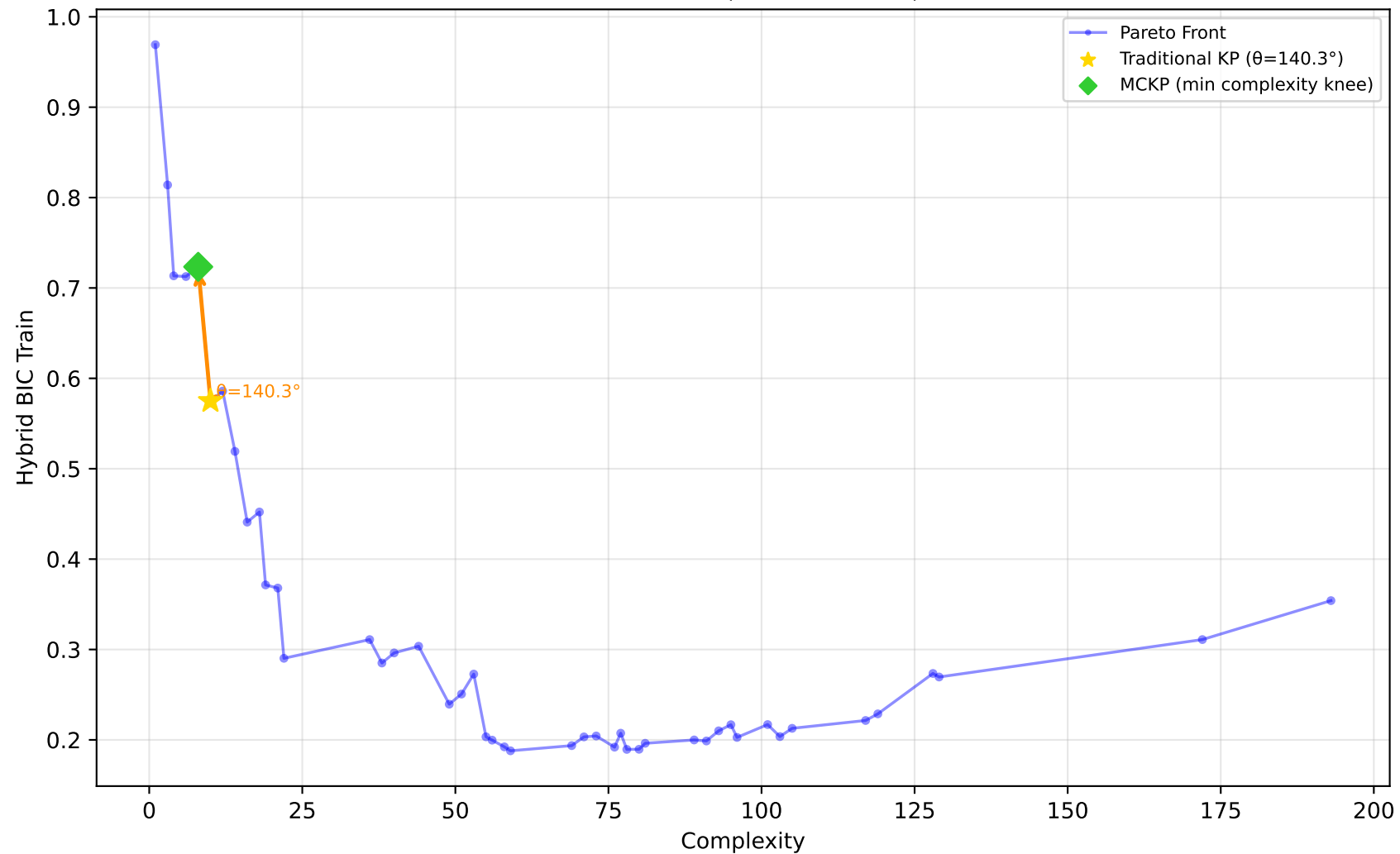
605_fri_c2_250_25 - Run 25 - MVP - Hybrid BIC Train \lambda_1=0.30, \lambda_2=0.00, \lambda_3=1.00 | Difficulty: 1.00 | Method: hmr
