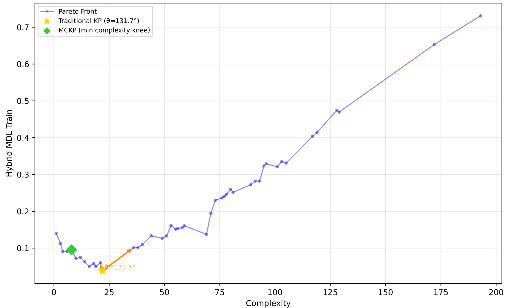
605_fri_c2_250_25 - Run 25 - MVP - Hybrid MDL Train \lambda_1=0.10, \lambda_2=0.00, \lambda_3=0.00 | Difficulty: 1.00 | Method: hmr
