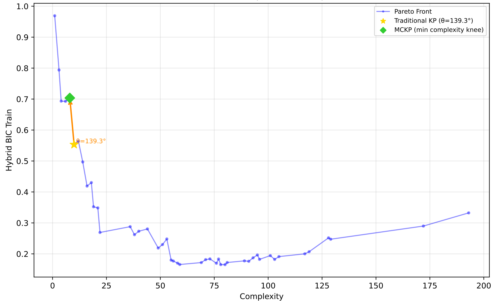
605_fri_c2_250_25 - Run 25 - SVP - Hybrid BIC Train \lambda_1=0.10, \lambda_2=0.00, \lambda_3=0.00 | Difficulty: 1.00 | Method: hmr
