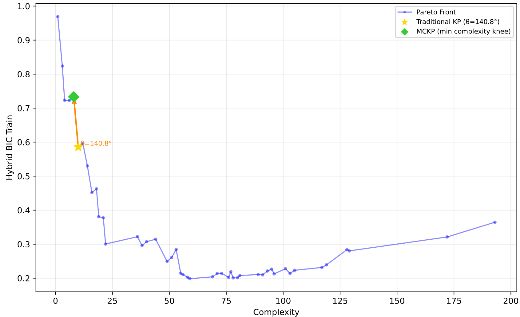
605_fri_c2_250_25 - Run 25 - SVP - Hybrid BIC Train \lambda_1=0.40, \lambda_2=0.00, \lambda_3=0.20 | Difficulty: 1.00 | Method: hmr
