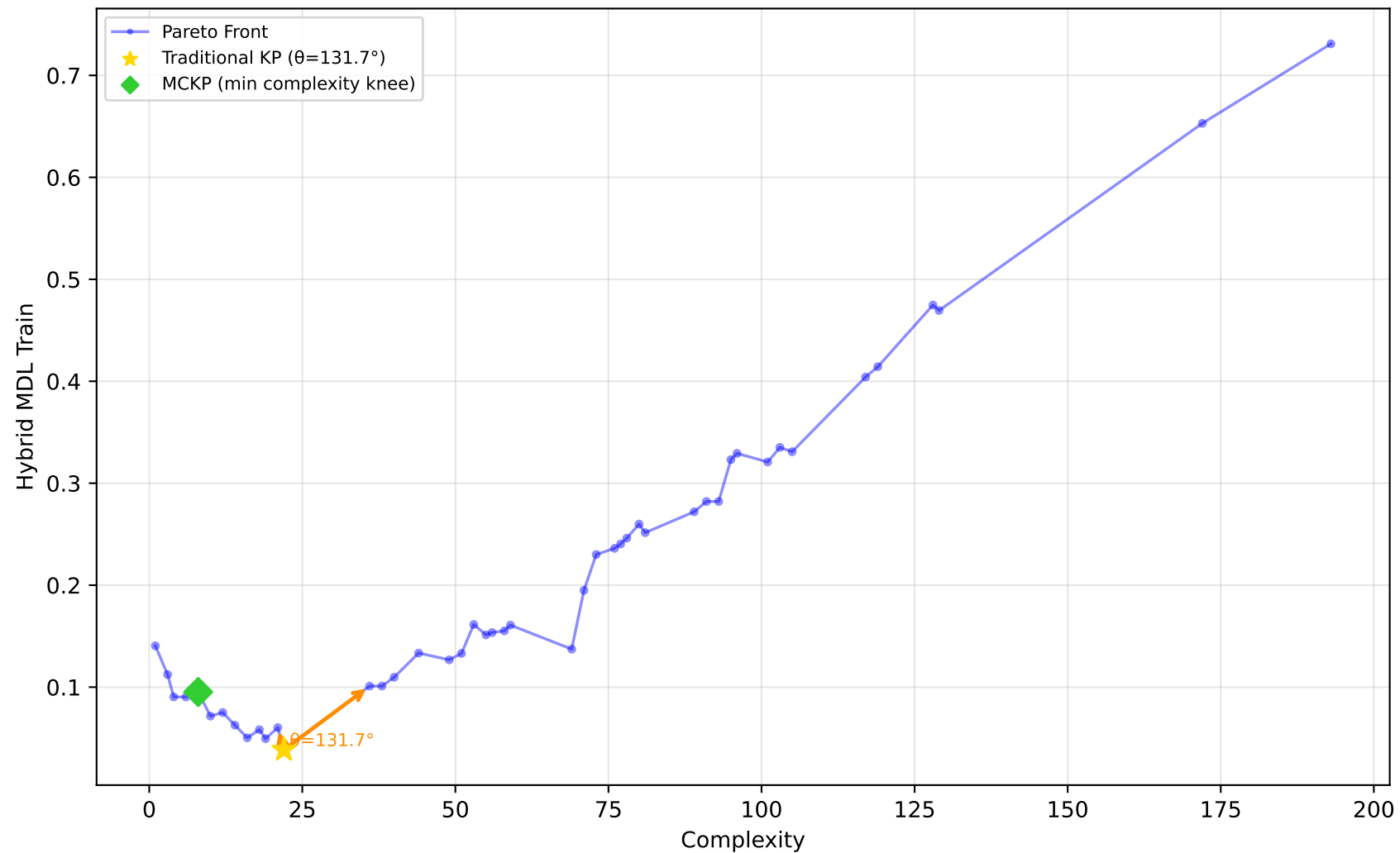
605_fri_c2_250_25 - Run 25 - SVP - Hybrid MDL Train \lambda_1=0.10, \bar{\lambda}_2=0.00, \bar{\lambda}_3=0.00 | Difficulty: 1.00 | Method: hmr
