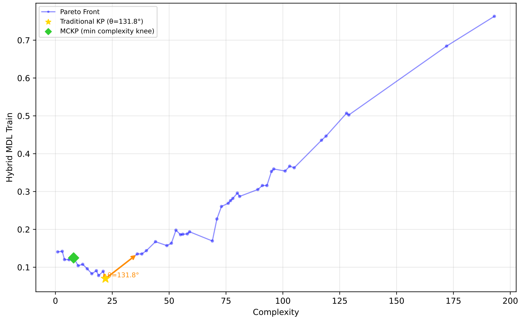
605_fri_c2_250_25 - Run 25 - SVP - Hybrid MDL Train \lambda_1=0.40, \lambda_2=0.00, \lambda_3=0.20 | Difficulty: 1.00 | Method: hmr
