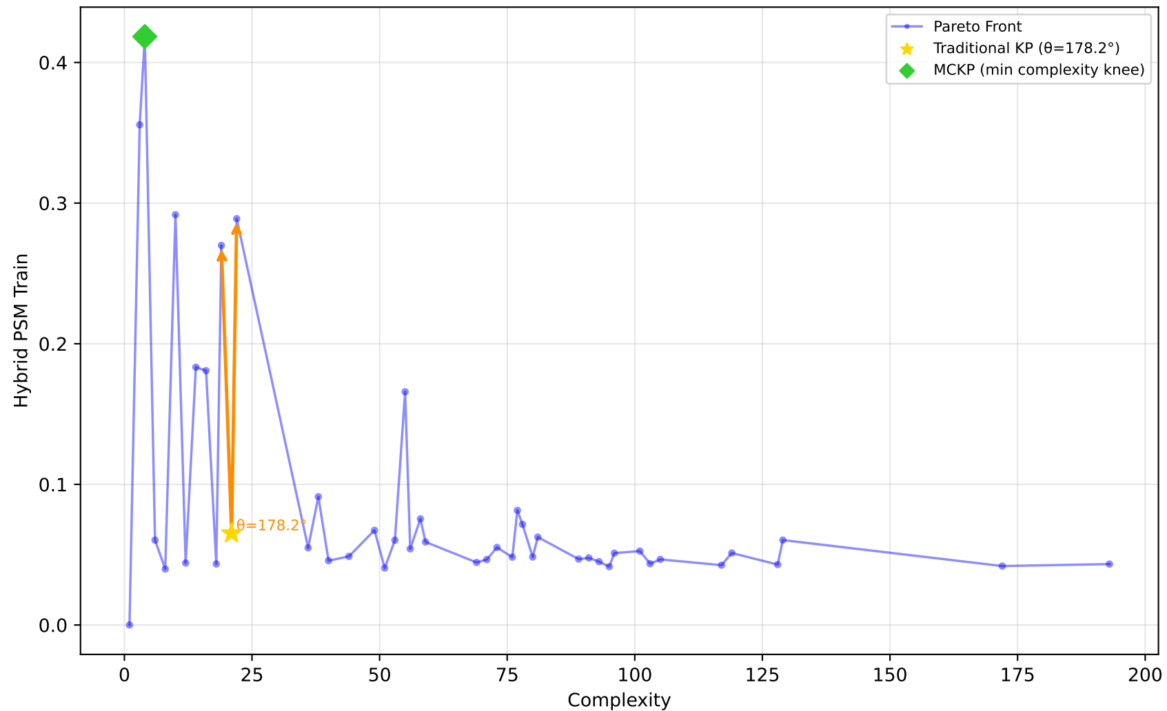
605_fri_c2_250_25 - Run 25 - SVP - Hybrid PSM Train \lambda_1=0.40, \bar{\lambda}_2=0.00, \bar{\lambda}_3=0.20 | Difficulty: 1.00 | Method: hmr
