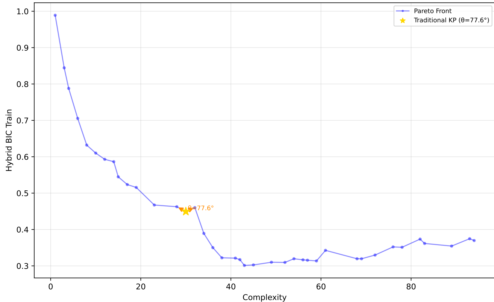
605_fri_c2_250_25 - Run 26 - MVP - Hybrid BIC Train \lambda_1=0.30, \lambda_2=0.00, \lambda_3=1.00 | Difficulty: 1.00 | Method: hmr
