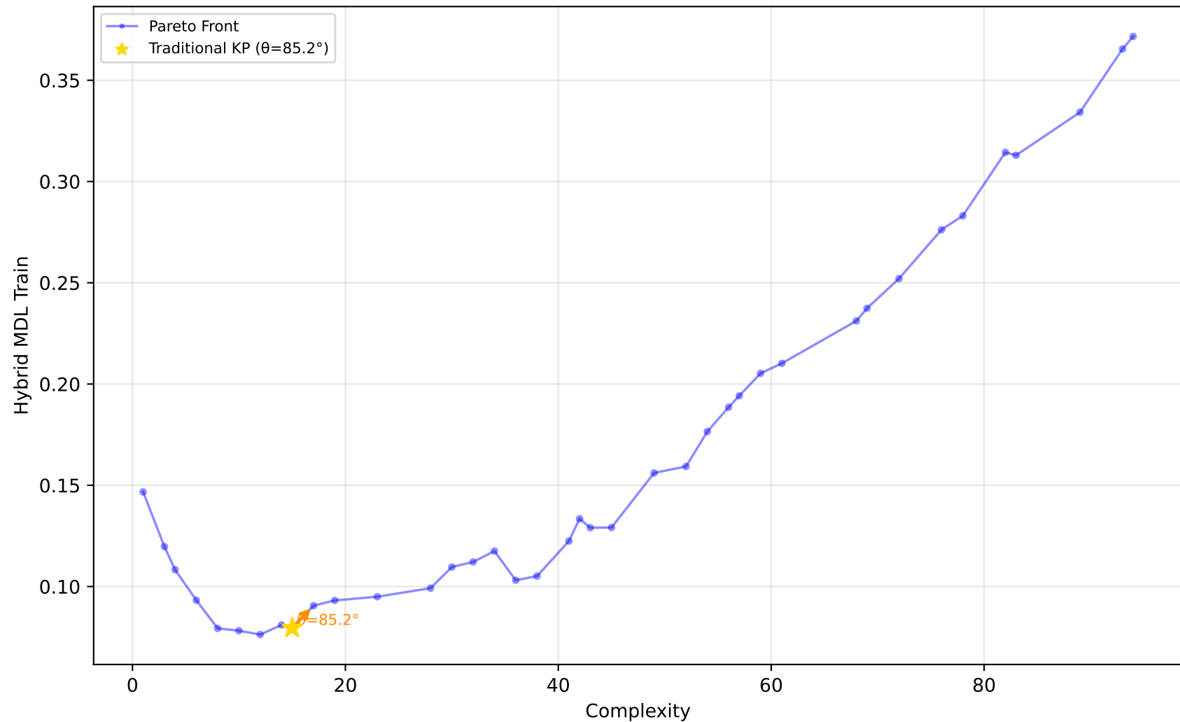
605_fri_c2_250_25 - Run 26 - MVP - Hybrid MDL Train \lambda_1=0.10 , \lambda_2=0.00 , \lambda_3=0.00 | Difficulty: 1.00 | Method: hmr
