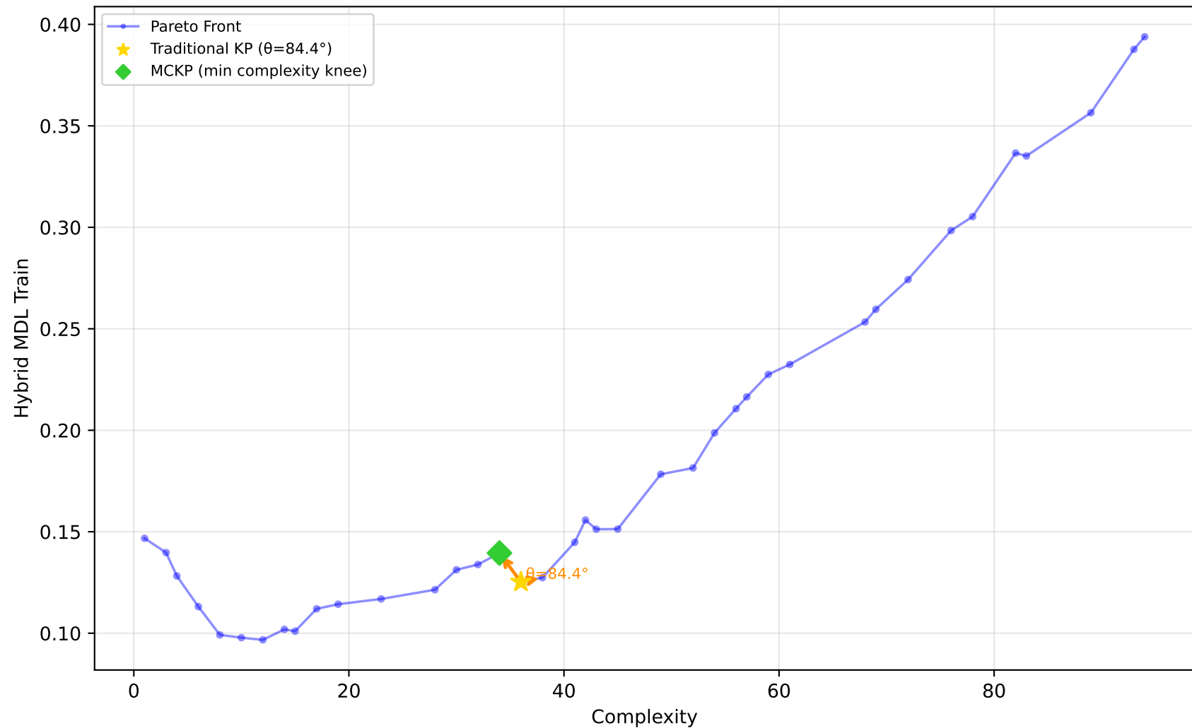
605_fri_c2_250_25 - Run 26 - MVP - Hybrid MDL Train \lambda_1=0.30, \lambda_2=0.00, \lambda_3=1.00 | Difficulty: 1.00 | Method: hmr
