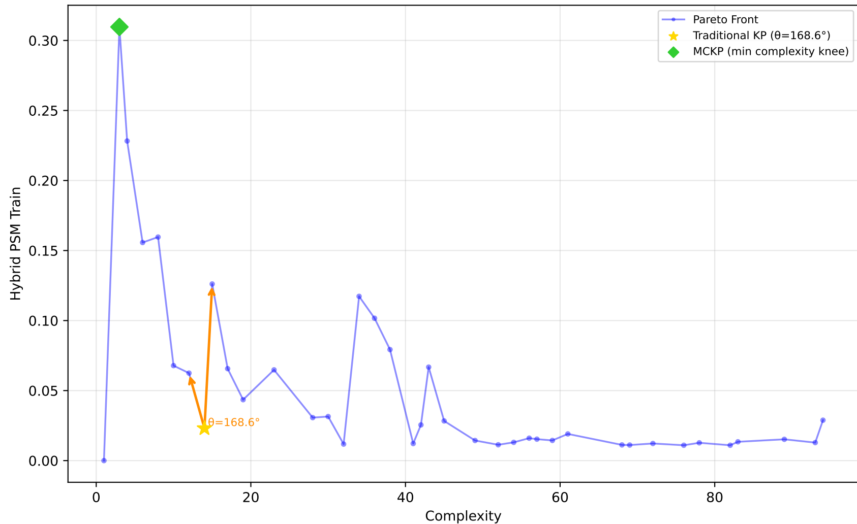
605_fri_c2_250_25 - Run 26 - MVP - Hybrid PSM Train \lambda_1=0.10, \lambda_2=0.00, \lambda_3=0.00 | Difficulty: 1.00 | Method: hmr
