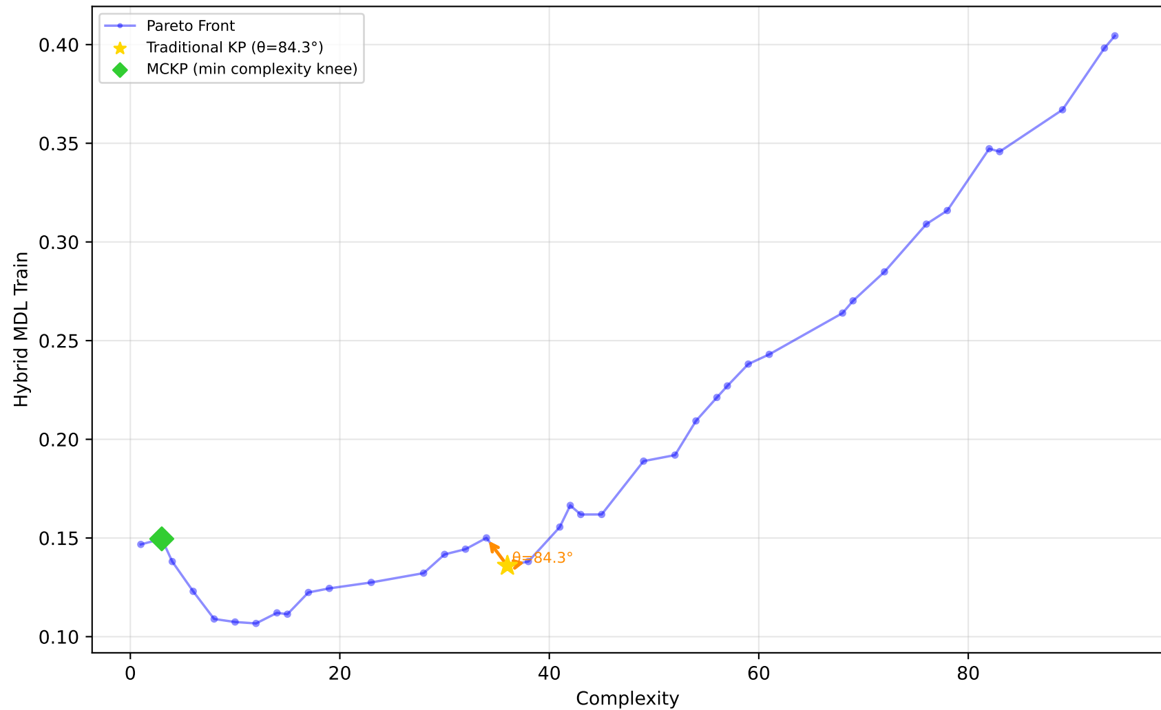
605_fri_c2_250_25 - Run 26 - SVP - Hybrid MDL Train \lambda_1=0.40 , \lambda_2=0.00 , \lambda_3=0.20 | Difficulty: 1.00 | Method: hmr
