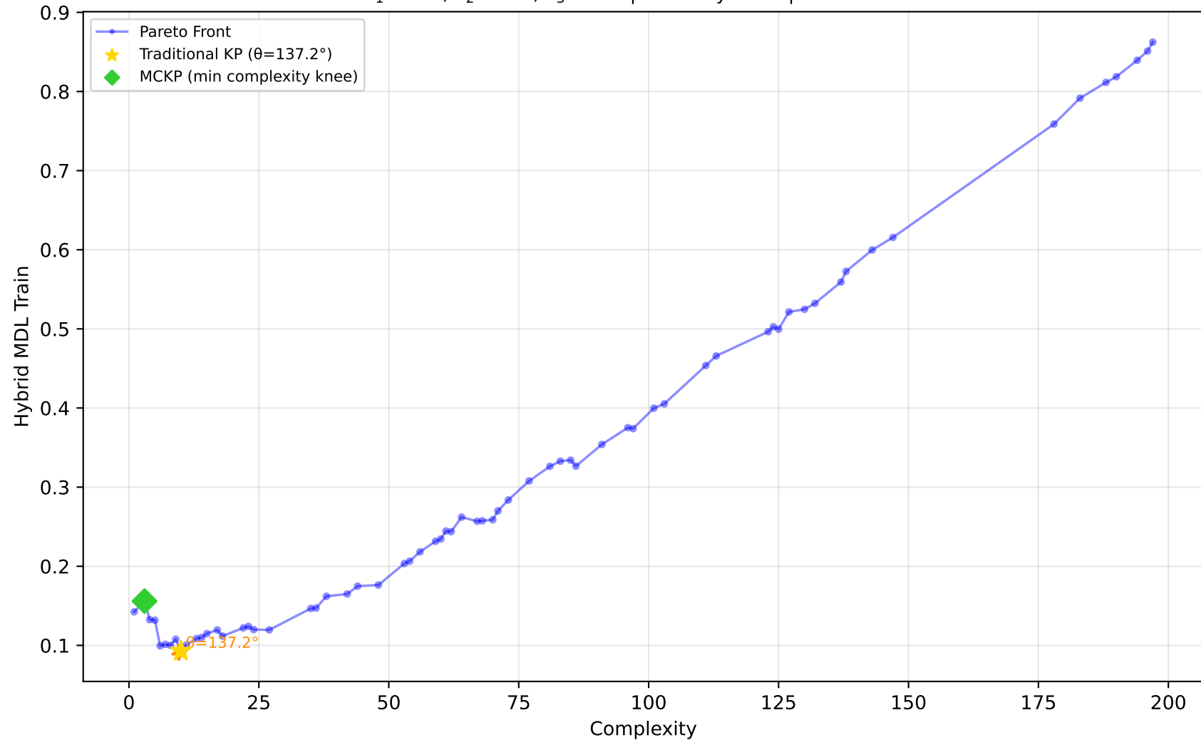
605_fri_c2_250_25 - Run 27 - MVP - Hybrid MDL Train \lambda_1=0.30, \bar{\lambda}_2=0.00, \lambda_3=1.00 | Difficulty: 1.00 | Method: hmr
