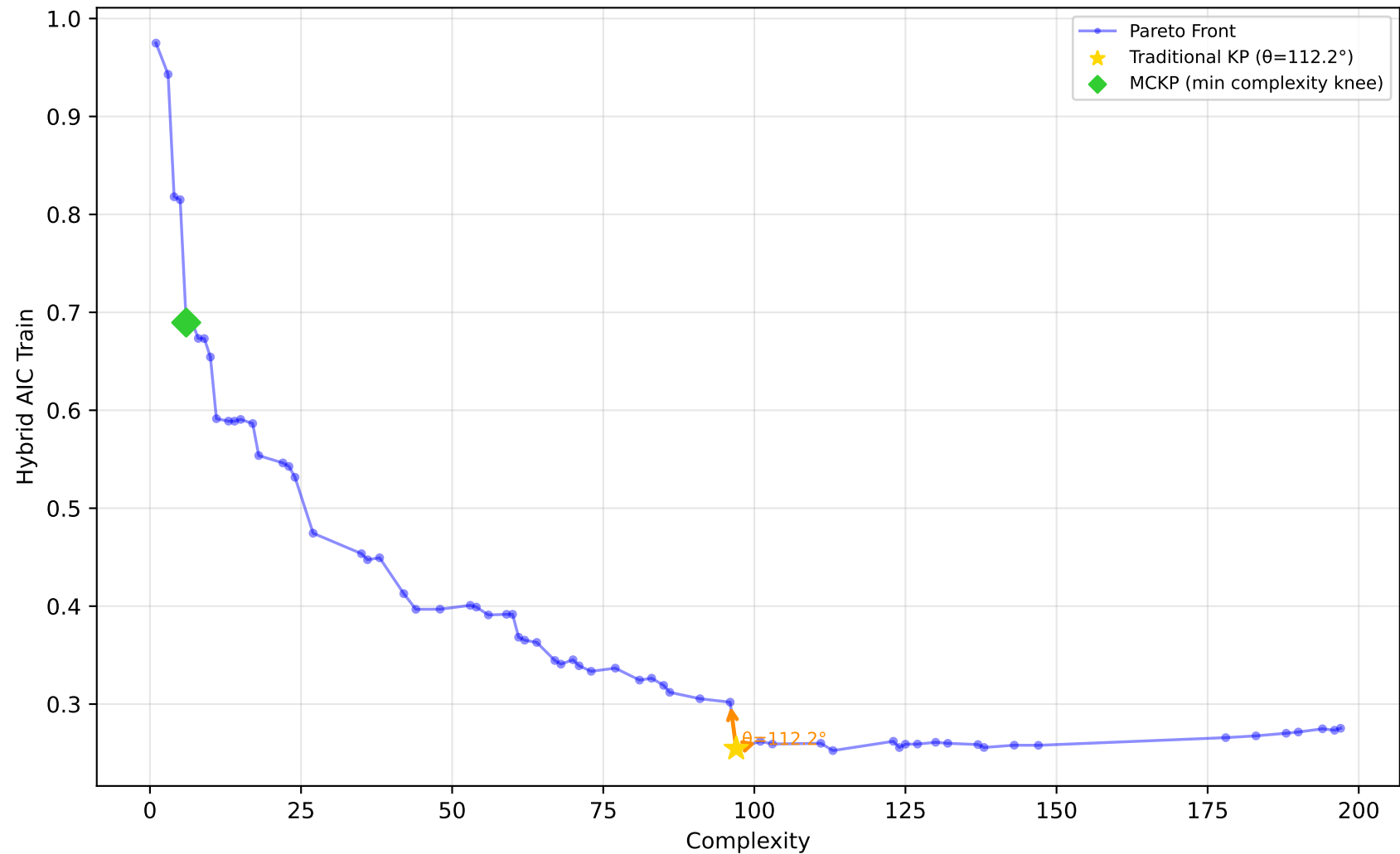
605_fri_c2_250_25 - Run 27 - SVP - Hybrid AIC Train \lambda_1=0.10, \lambda_2=0.00, \lambda_3=0.00 | Difficulty: 1.00 | Method: hmr
