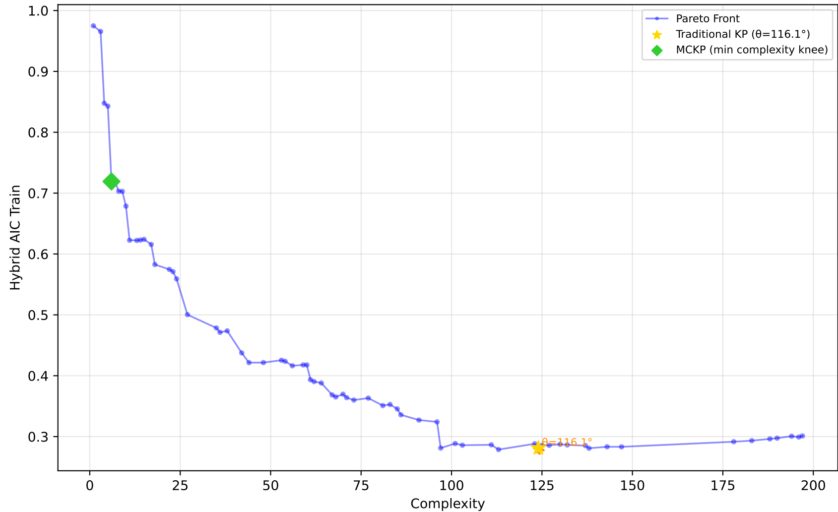
605_fri_c2_250_25 - Run 27 - SVP - Hybrid AIC Train \lambda_1=0.40 , \lambda_2=0.00 , \lambda_3=0.20 | Difficulty: 1.00 | Method: hmr
