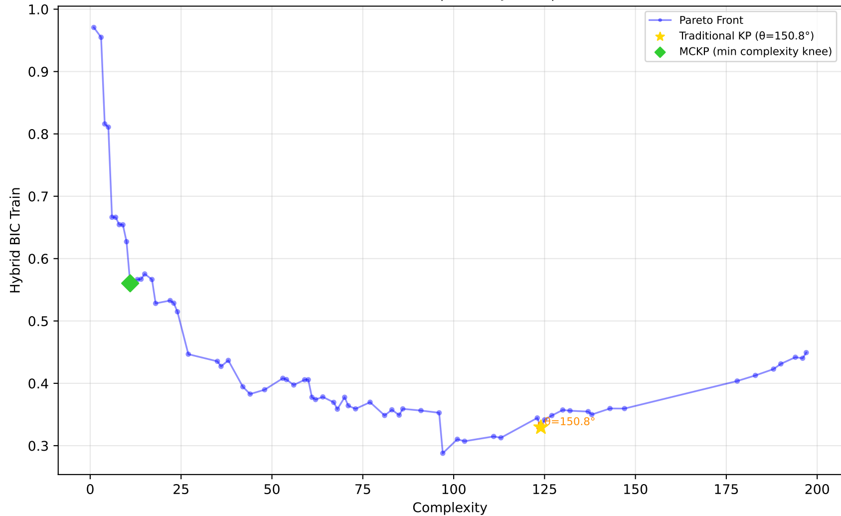
605_fri_c2_250_25 - Run 27 - SVP - Hybrid BIC Train \lambda_1=0.40 , \lambda_2=0.00 , \lambda_3=0.20 | Difficulty: 1.00 | Method: hmr
