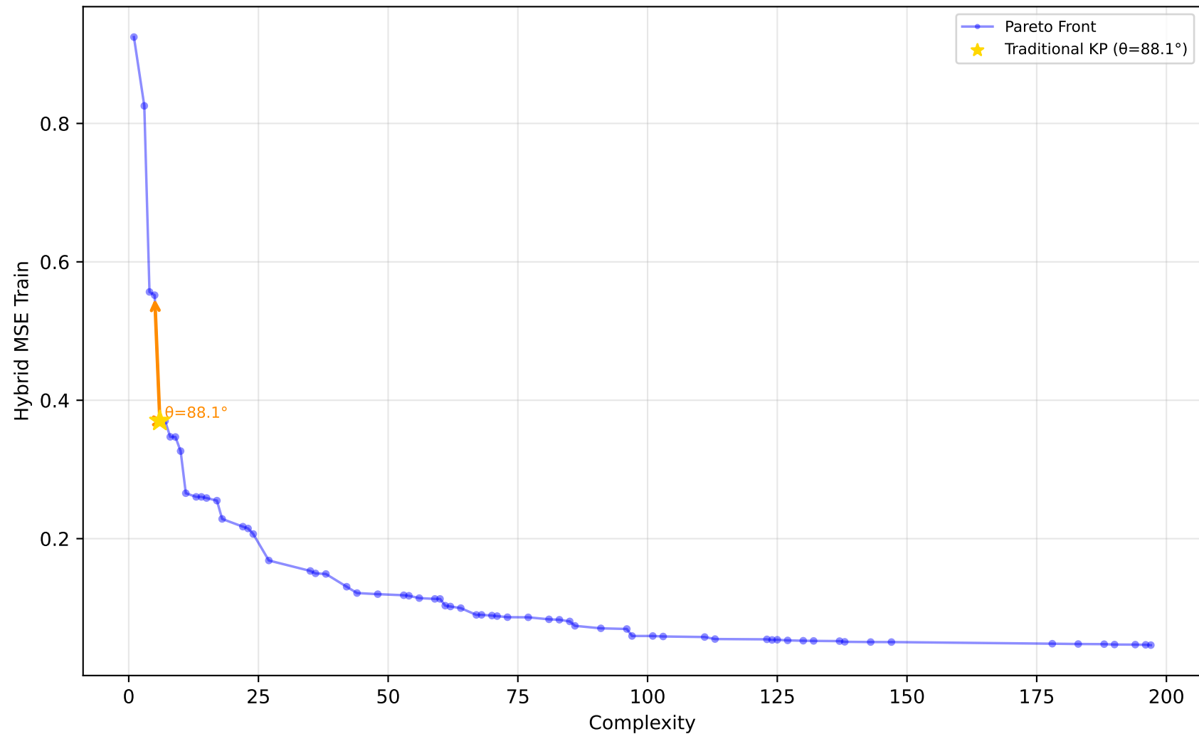
605_fri_c2_250_25 - Run 27 - SVP - Hybrid MSE Train \lambda_1=0.10, \lambda_2=0.00, \lambda_3=0.00 | Difficulty: 1.00 | Method: hmr
