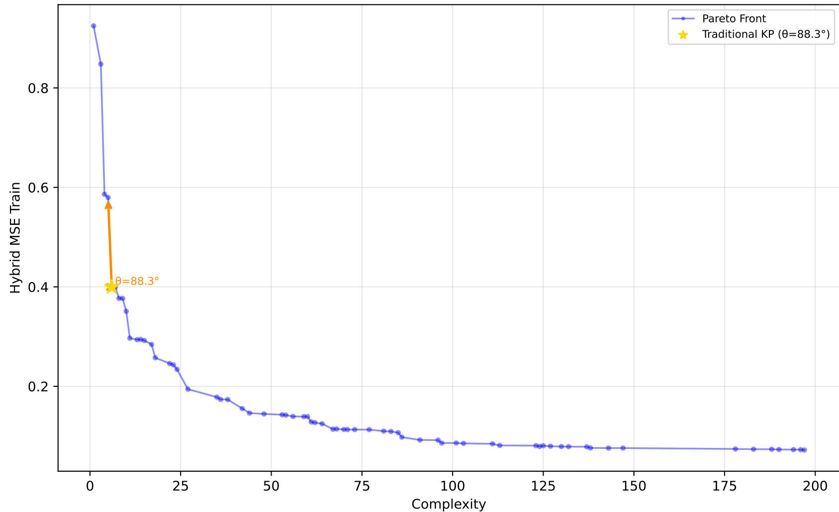
605_fri_c2_250_25 - Run 27 - SVP - Hybrid MSE Train \lambda_1=0.40, \lambda_2=0.00, \lambda_3=0.20 | Difficulty: 1.00 | Method: hmr
