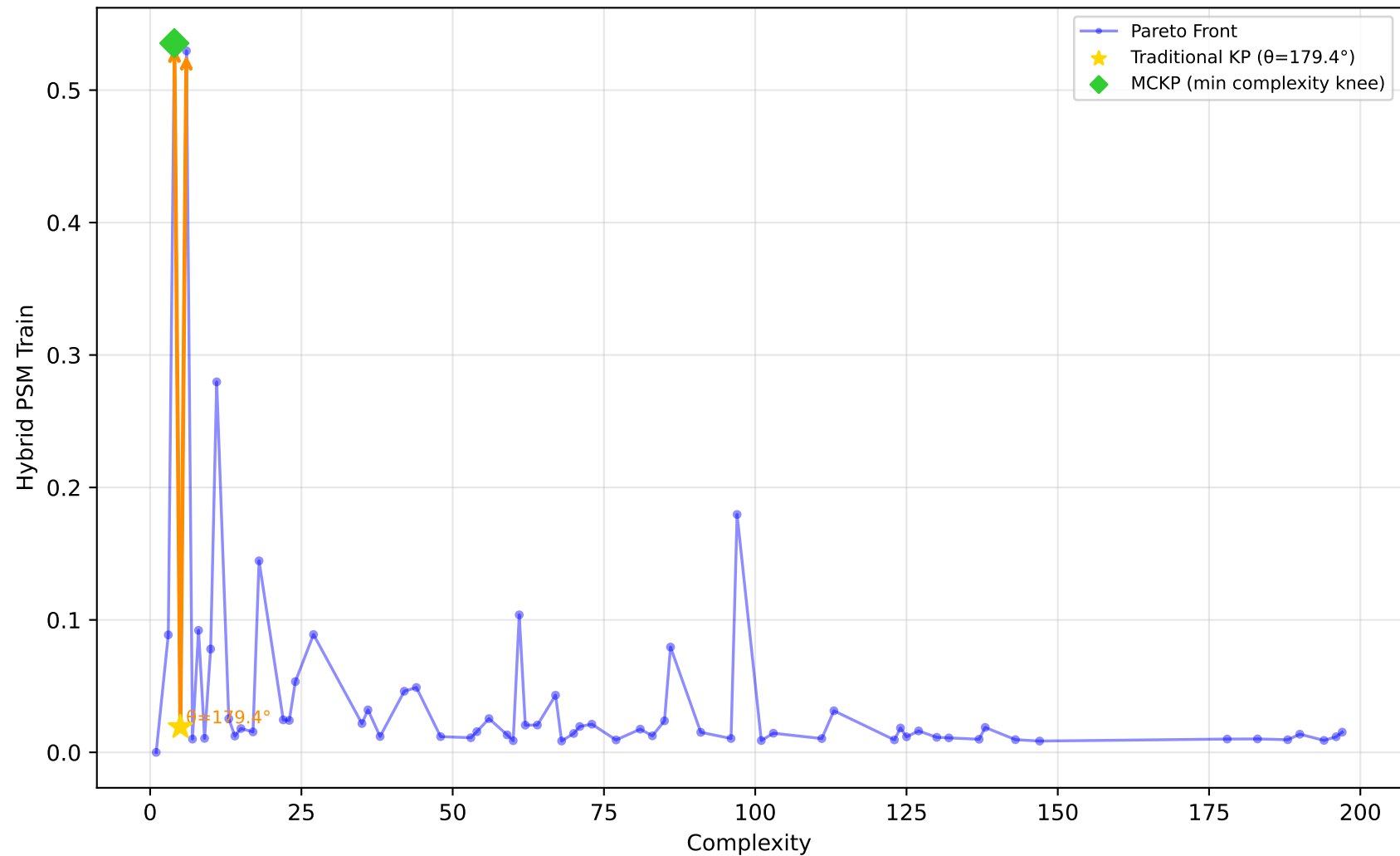
605_fri_c2_250_25 - Run 27 - SVP - Hybrid PSM Train \lambda_1=0.10, \lambda_2=0.00, \lambda_3=0.00 | Difficulty: 1.00 | Method: hmr
