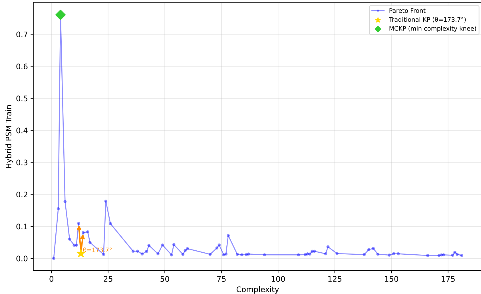
605_fri_c2_250_25 - Run 28 - MVP - Hybrid PSM Train \lambda_1=0.10, \bar{\lambda}_2=0.00, \bar{\lambda}_3=0.00 | Difficulty: 1.00 | Method: hmr
