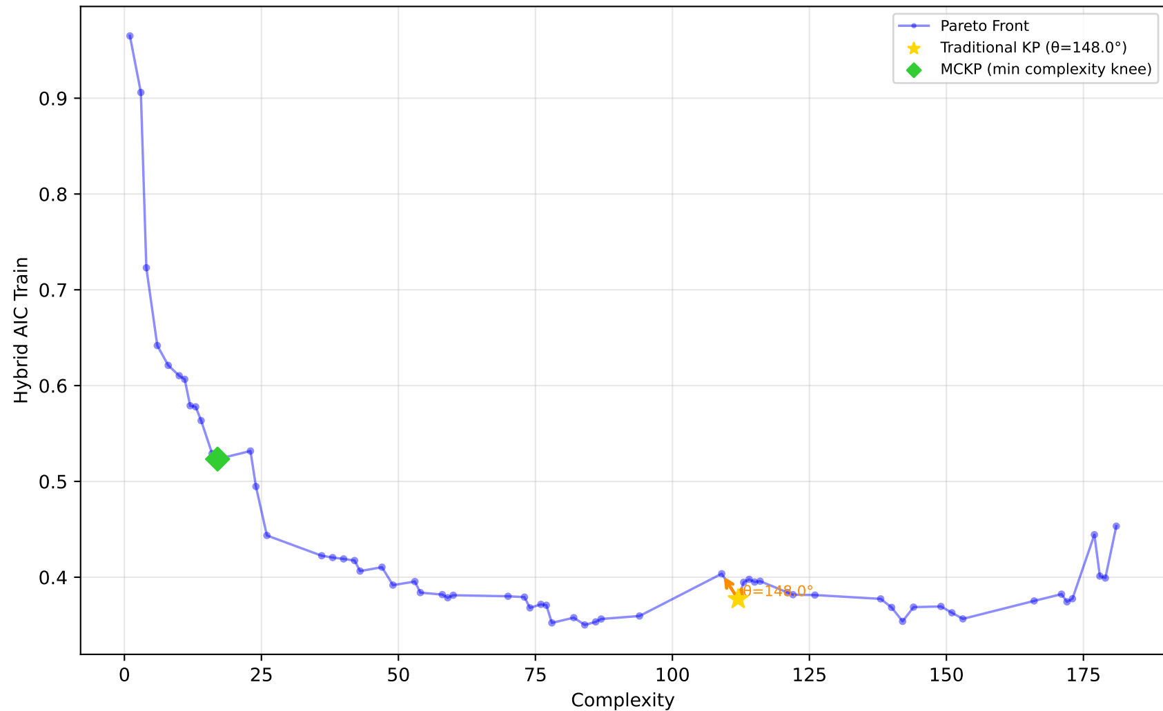
605_fri_c2_250_25 - Run 28 - SVP - Hybrid AIC Train \lambda_1=0.10, \lambda_2=0.00, \lambda_3=0.00 | Difficulty: 1.00 | Method: hmr
