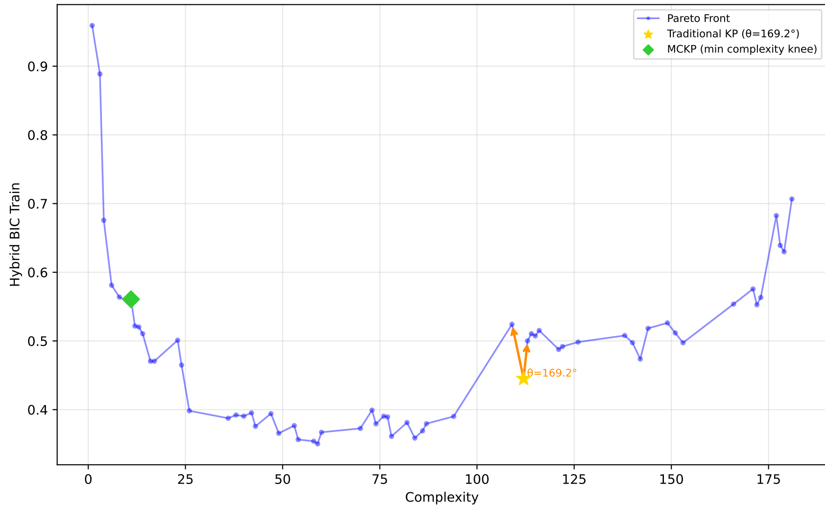
605_fri_c2_250_25 - Run 28 - SVP - Hybrid BIC Train \lambda_1=0.10, \lambda_2=0.00, \lambda_3=0.00 | Difficulty: 1.00 | Method: hmr
