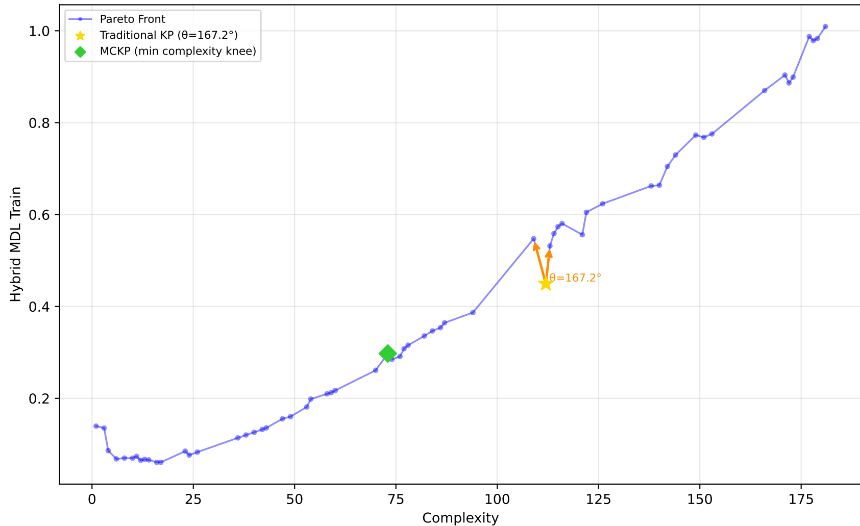
605_fri_c2_250_25 - Run 28 - SVP - Hybrid MDL Train \lambda_1=0.10, \bar{\lambda}_2=0.00, \bar{\lambda}_3=0.00 | Difficulty: 1.00 | Method: hmr
