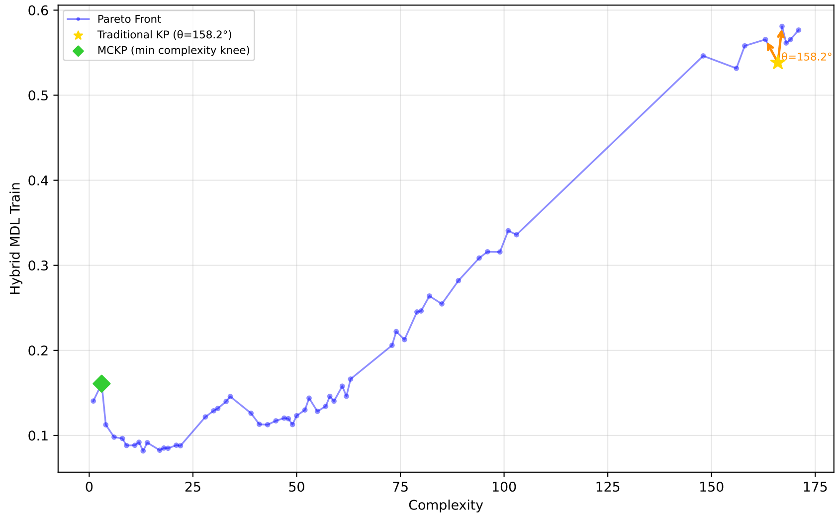
605_fri_c2_250_25 - Run 29 - MVP - Hybrid MDL Train \lambda_1=0.30, \lambda_2=0.00, \lambda_3=1.00 | Difficulty: 1.00 | Method: hmr
