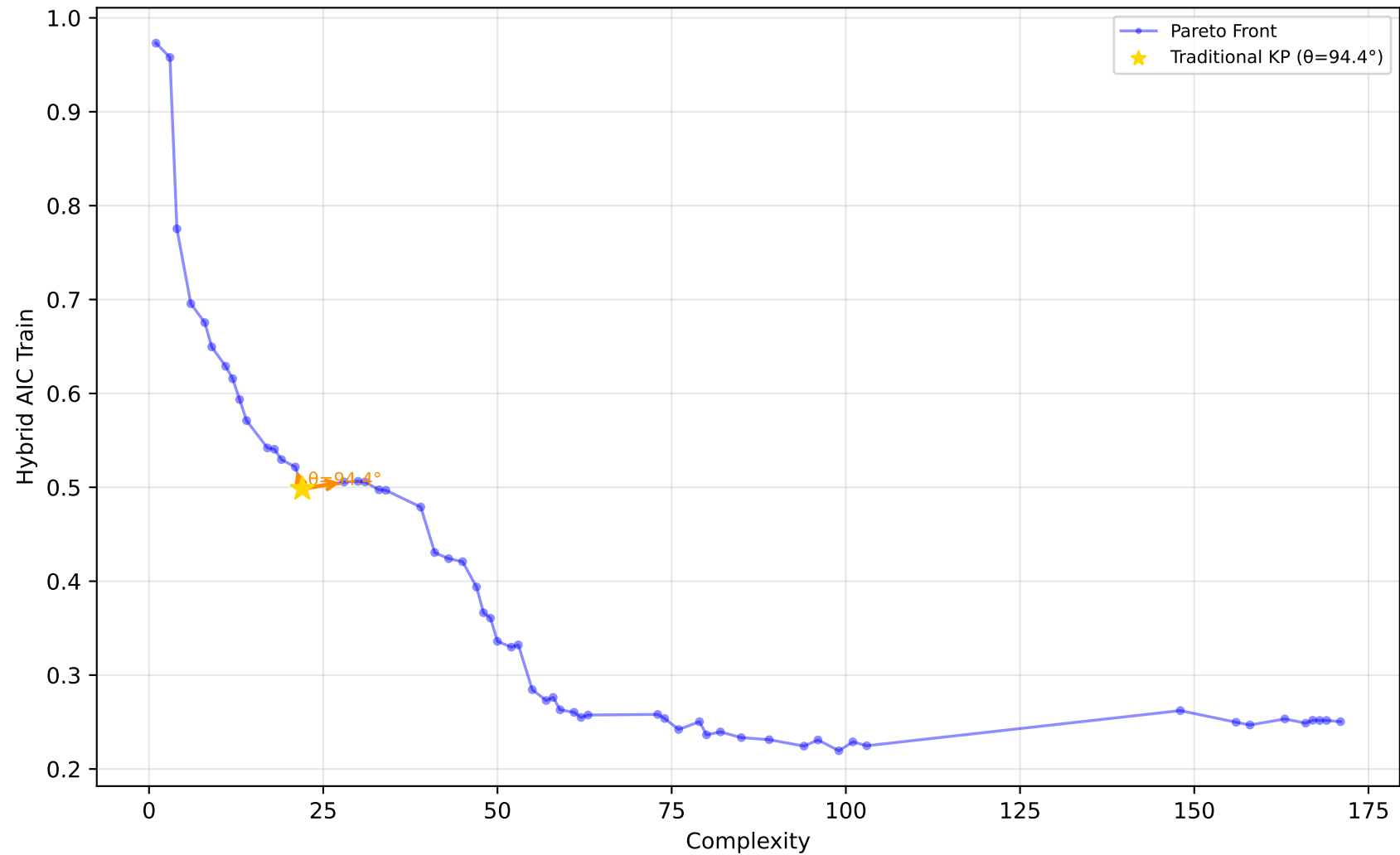
605_fri_c2_250_25 - Run 29 - SVP - Hybrid AIC Train \lambda_1=0.40, \lambda_2=0.00, \lambda_3=0.20 | Difficulty: 1.00 | Method: hmr
