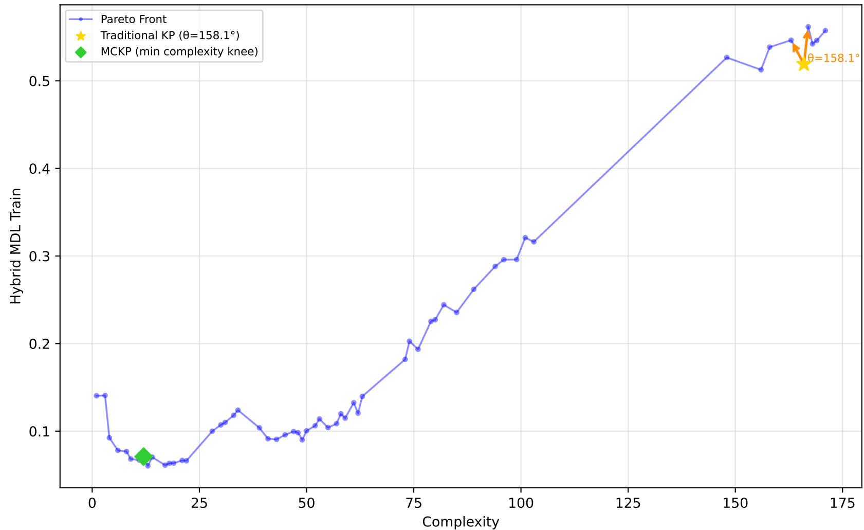
605_fri_c2_250_25 - Run 29 - SVP - Hybrid MDL Train \lambda_1=0.10, \lambda_2=0.00, \lambda_3=0.00 | Difficulty: 1.00 | Method: hmr
