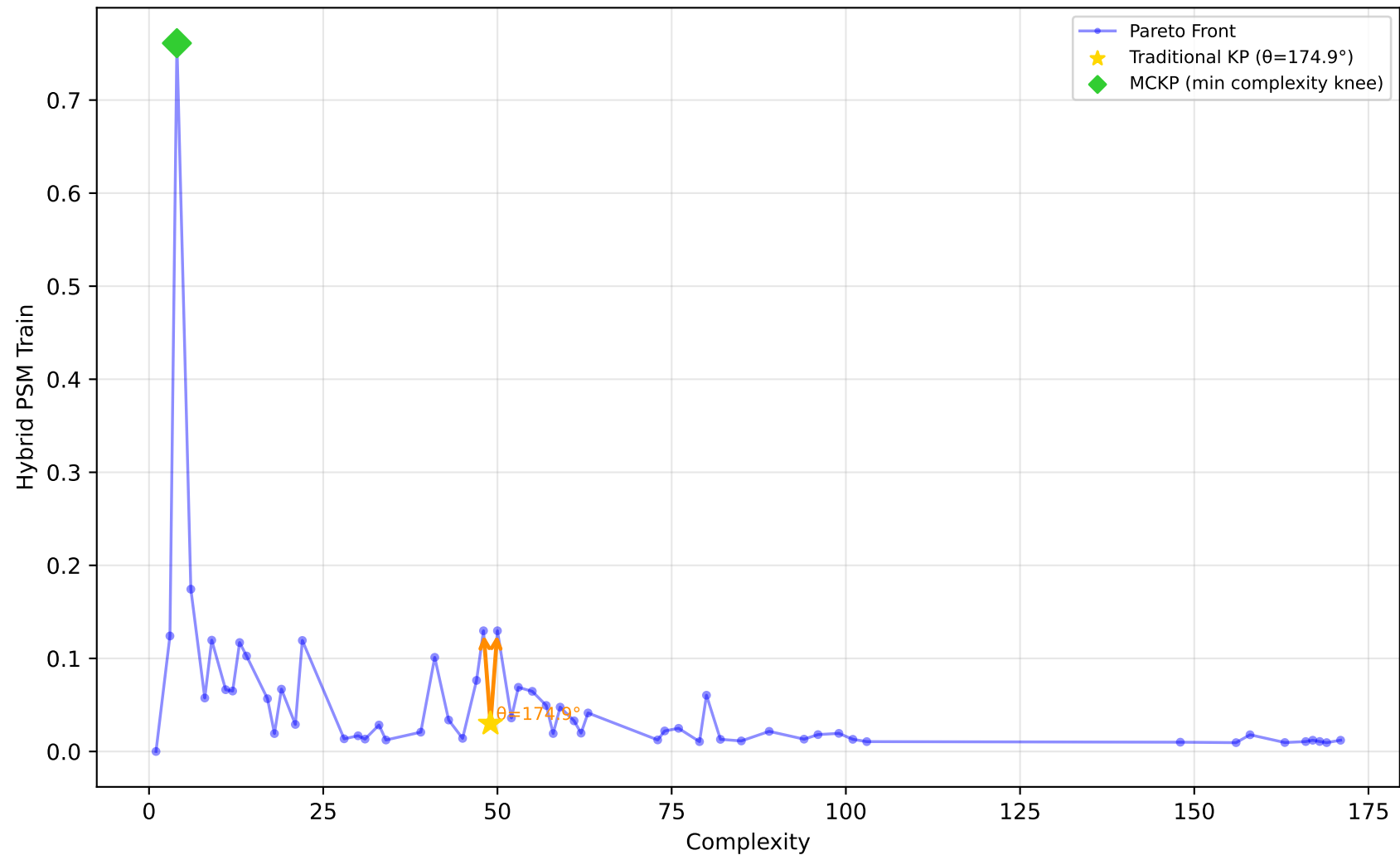
605_fri_c2_250_25 - Run 29 - SVP - Hybrid PSM Train \lambda_1=0.10, \lambda_2=0.00, \lambda_3=0.00 | Difficulty: 1.00 | Method: hmr
