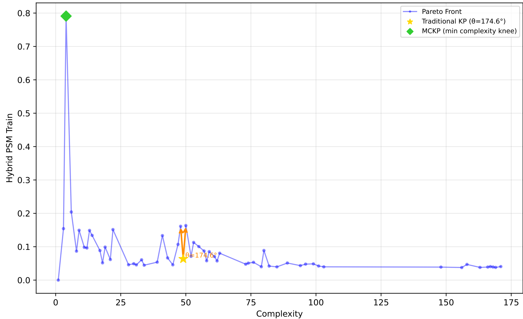
605_fri_c2_250_25 - Run 29 - SVP - Hybrid PSM Train \lambda_1=0.40, \lambda_2=0.00, \lambda_3=0.20 | Difficulty: 1.00 | Method: hmr
