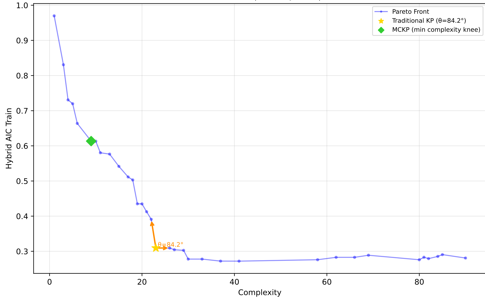
605_fri_c2_250_25 - Run 2 - MVP - Hybrid AIC Train \lambda_1=0.10, \lambda_2=0.00, \lambda_3=0.00 | Difficulty: 1.00 | Method: hmr
