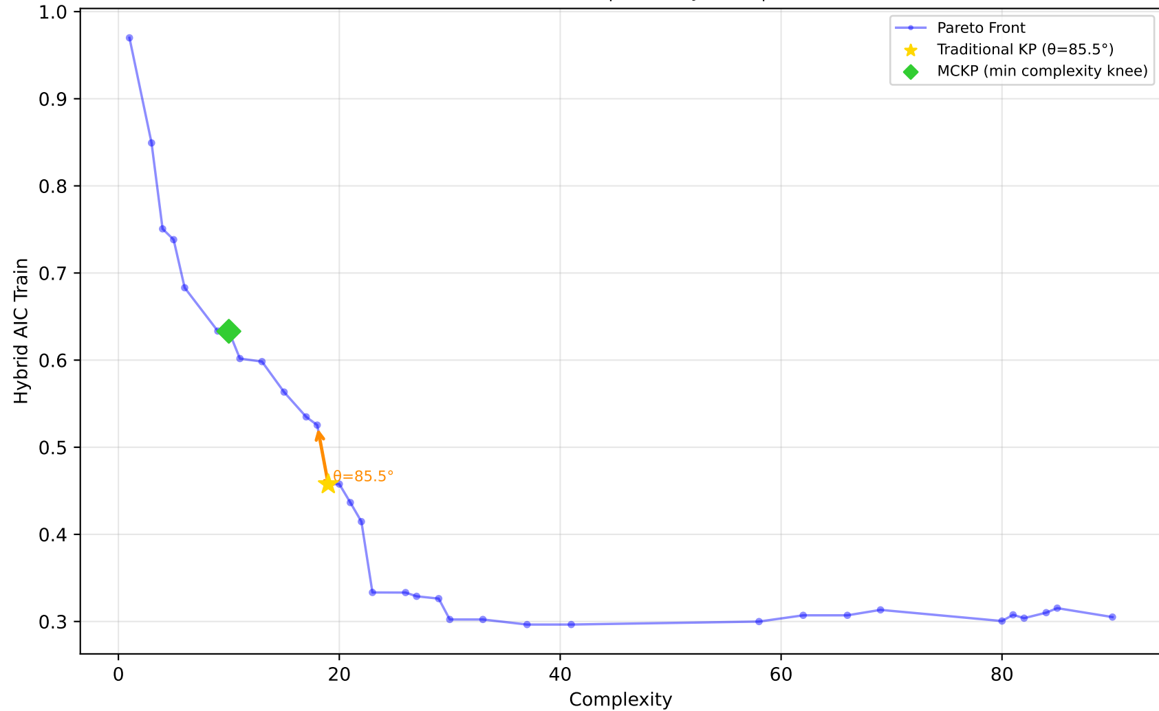
605_fri_c2_250_25 - Run 2 - MVP - Hybrid AIC Train \lambda_1=0.30, \lambda_2=0.00, \lambda_3=1.00 | Difficulty: 1.00 | Method: hmr
