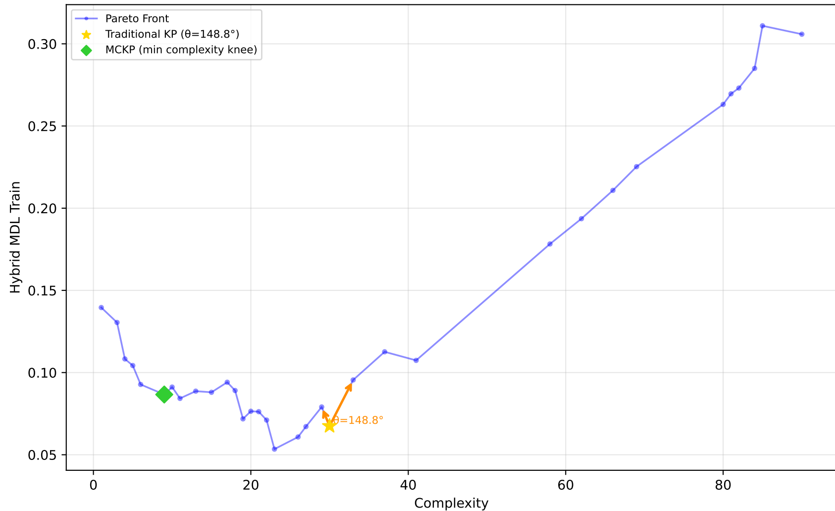
605_fri_c2_250_25 - Run 2 - MVP - Hybrid MDL Train \lambda_1=0.30 , \lambda_2=0.00 , \lambda_3=1.00 | Difficulty: 1.00 | Method: hmr
