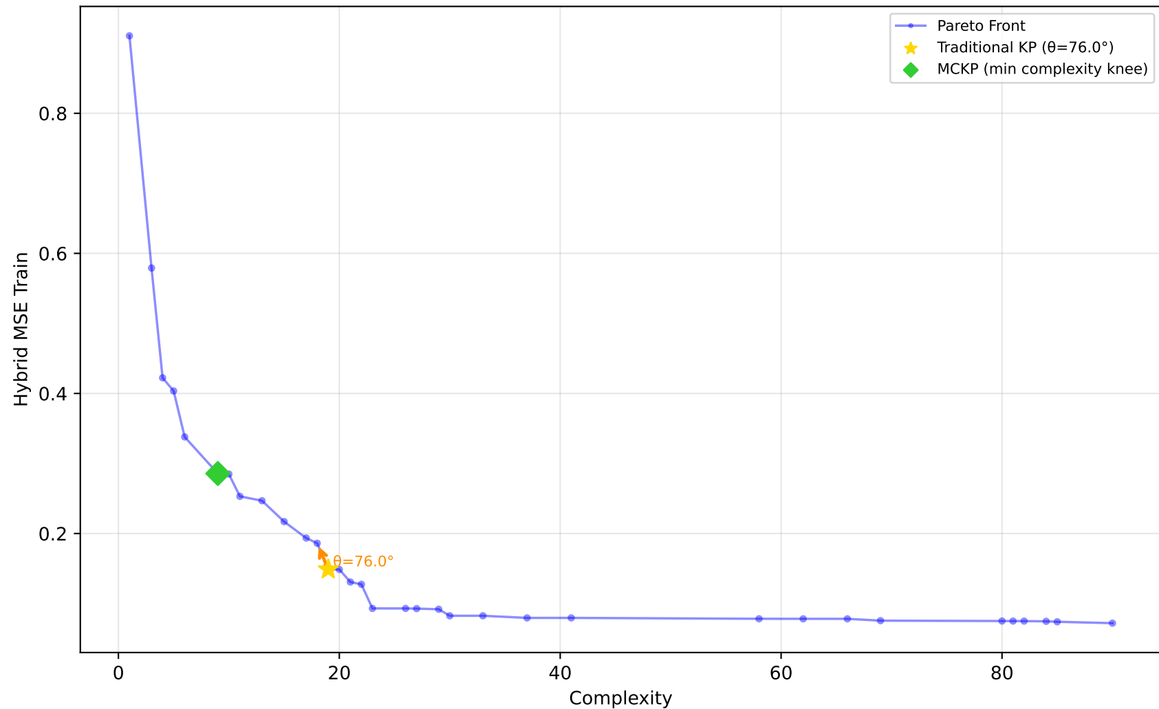
605_fri_c2_250_25 - Run 2 - MVP - Hybrid MSE Train \lambda_1=0.10, \lambda_2=0.00, \lambda_3=0.00 | Difficulty: 1.00 | Method: hmr
