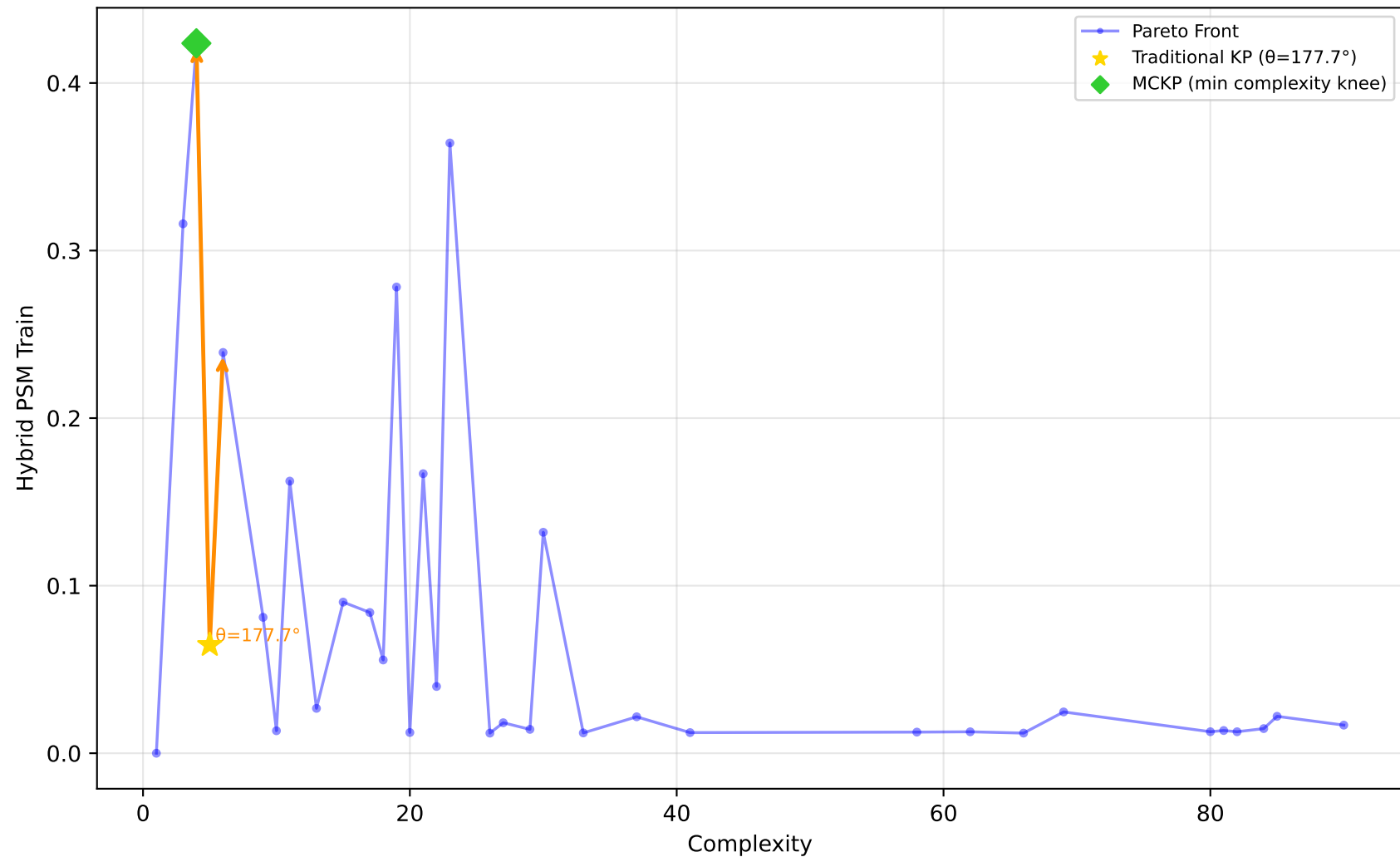
605_fri_c2_250_25 - Run 2 - SVP - Hybrid PSM Train \lambda_1=0.10, \lambda_2=0.00, \lambda_3=0.00 | Difficulty: 1.00 | Method: hmr
